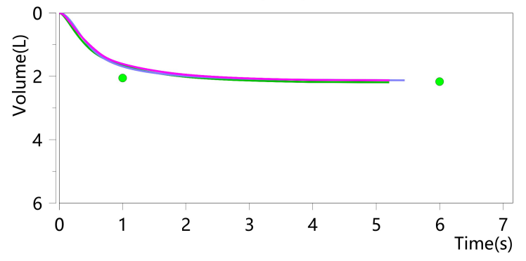
V-T(after)
