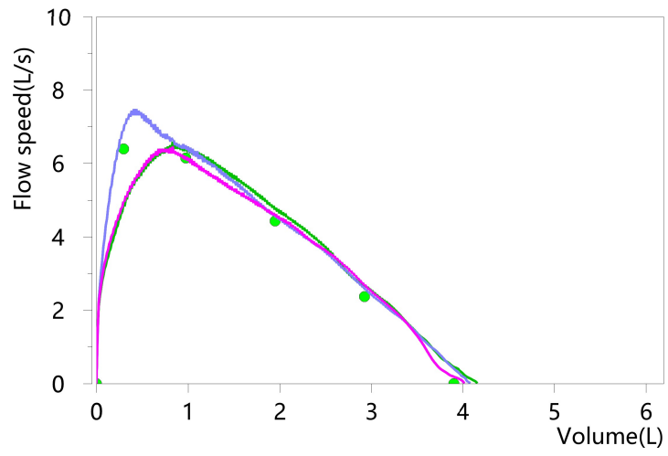
F-V(after)
